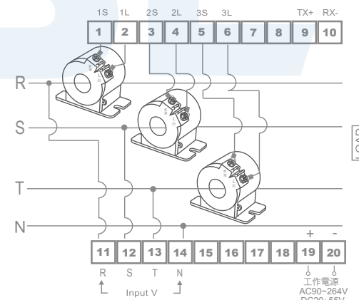
Model: 3Φ 4W (3CT)
