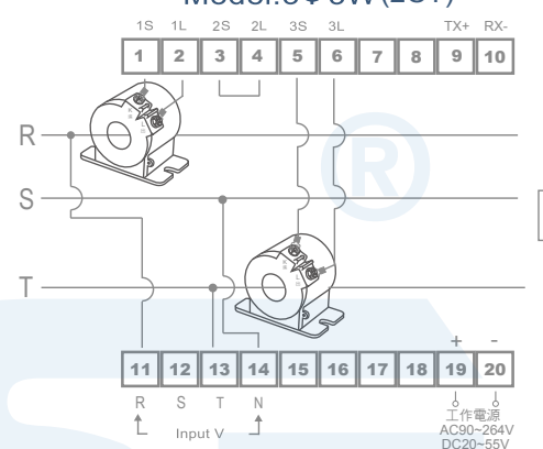
Model: 3Φ 3W (2CT)
